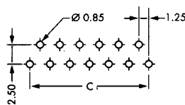
Recommended PC Board Pattern
