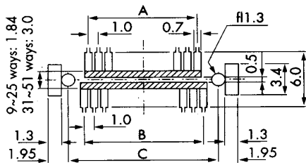
Surface Mount Plug
